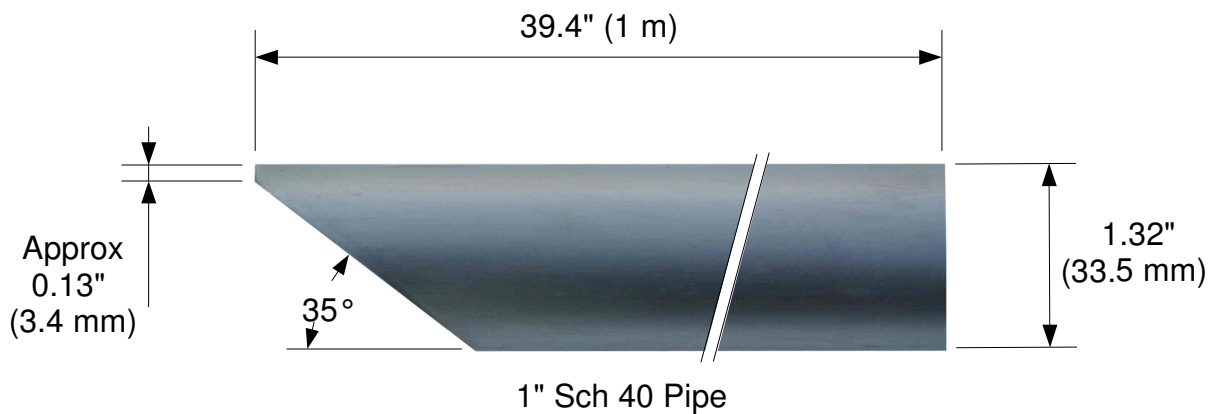
Image 2: Mounting Pipe Dimensions
