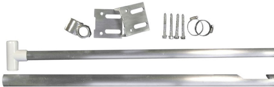
Image 1: KIT-PWRPOLEMNT components.
