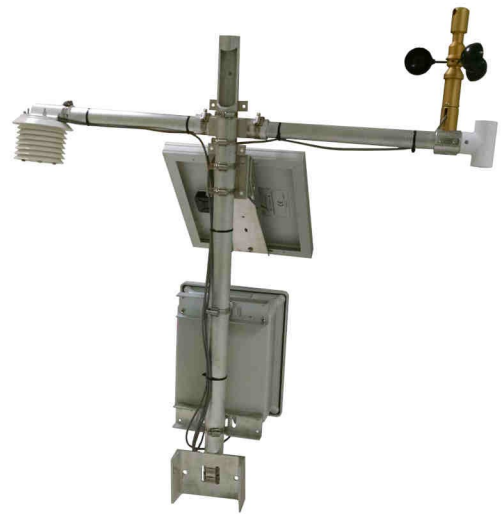
Step 2: Attach weather station components and bottom bracket to mast.
