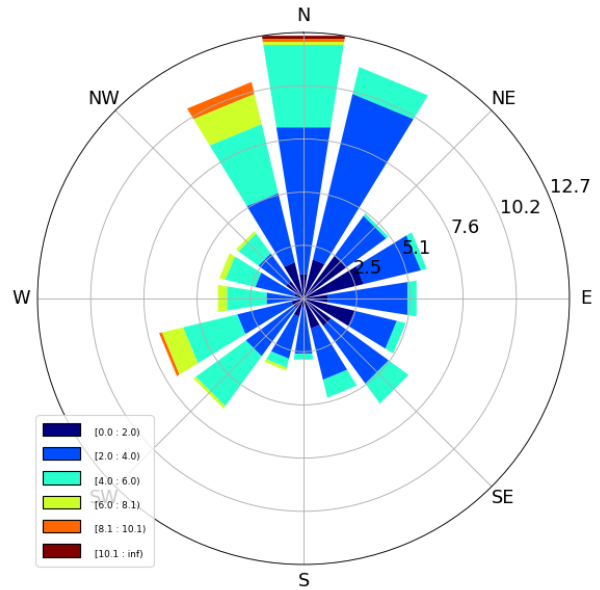
Wind Statistics
